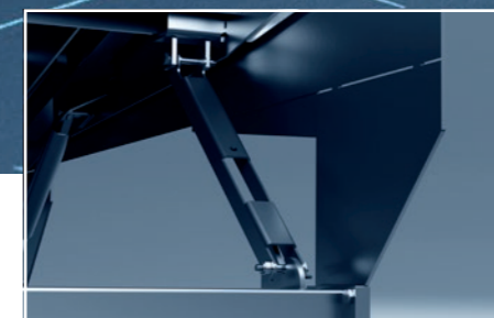
4. Self-positioning safety props improve both operational and maintenance safety, and can be put in position by one person in two simple steps
